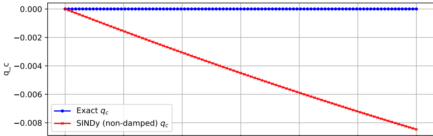
Trajectory 1890 (non-damped)
