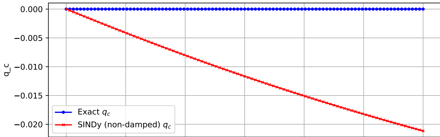
Trajectory 1891 (non-damped)
