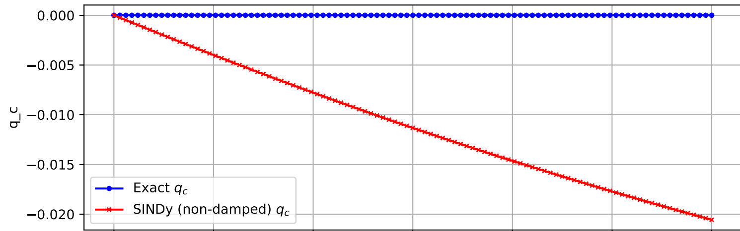
Trajectory 1893 (non-damped)
