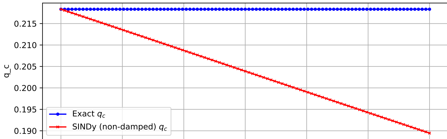
Trajectory 1901 (non-damped)
