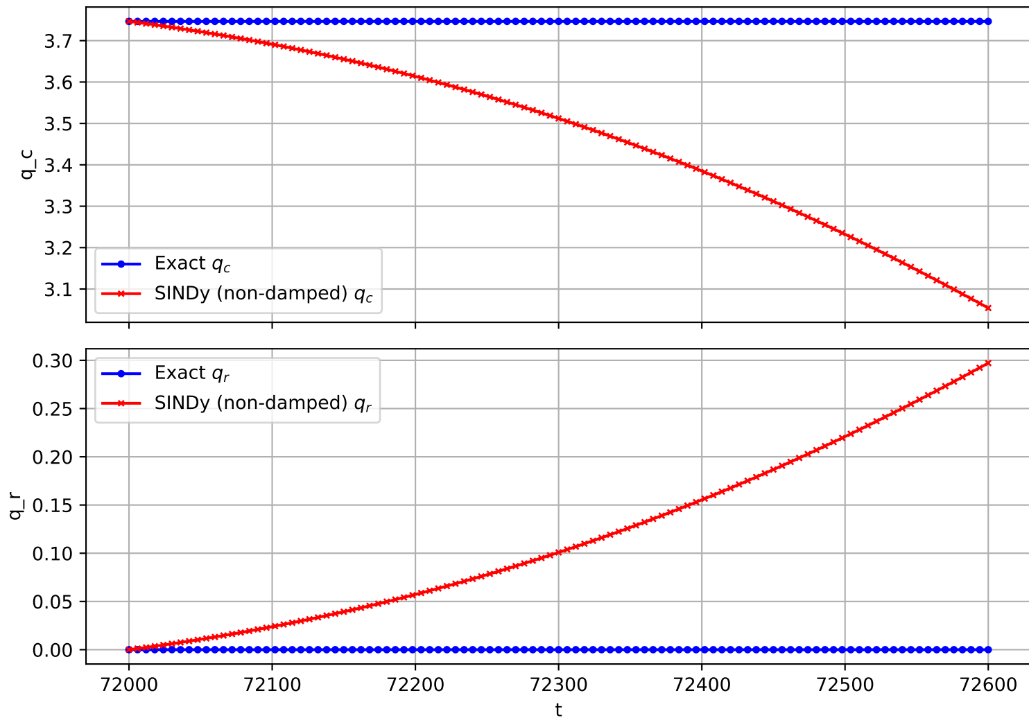
Trajectory 1903 (non-damped)
