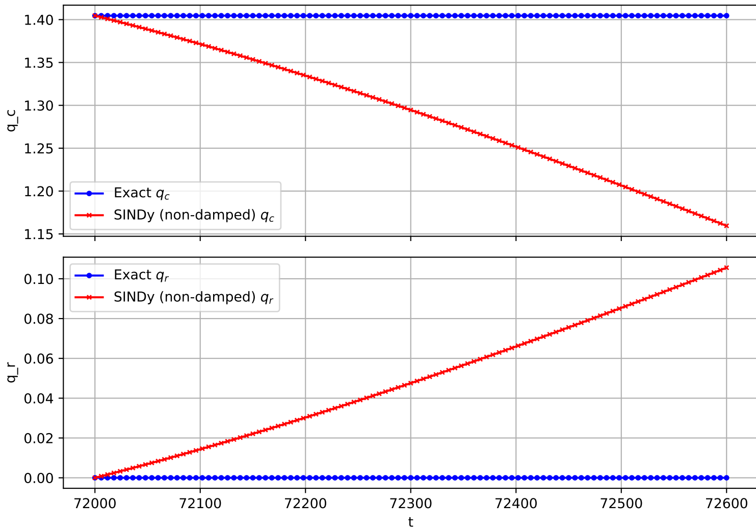
Trajectory 1907 (non-damped)
