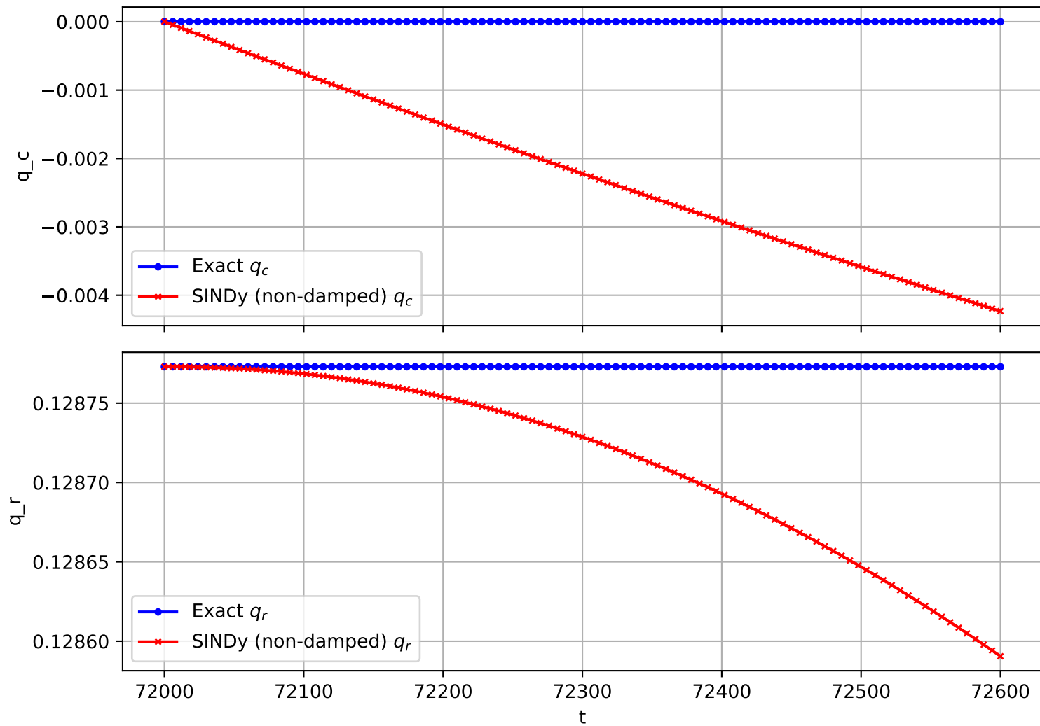
Trajectory 1911 (non-damped)
