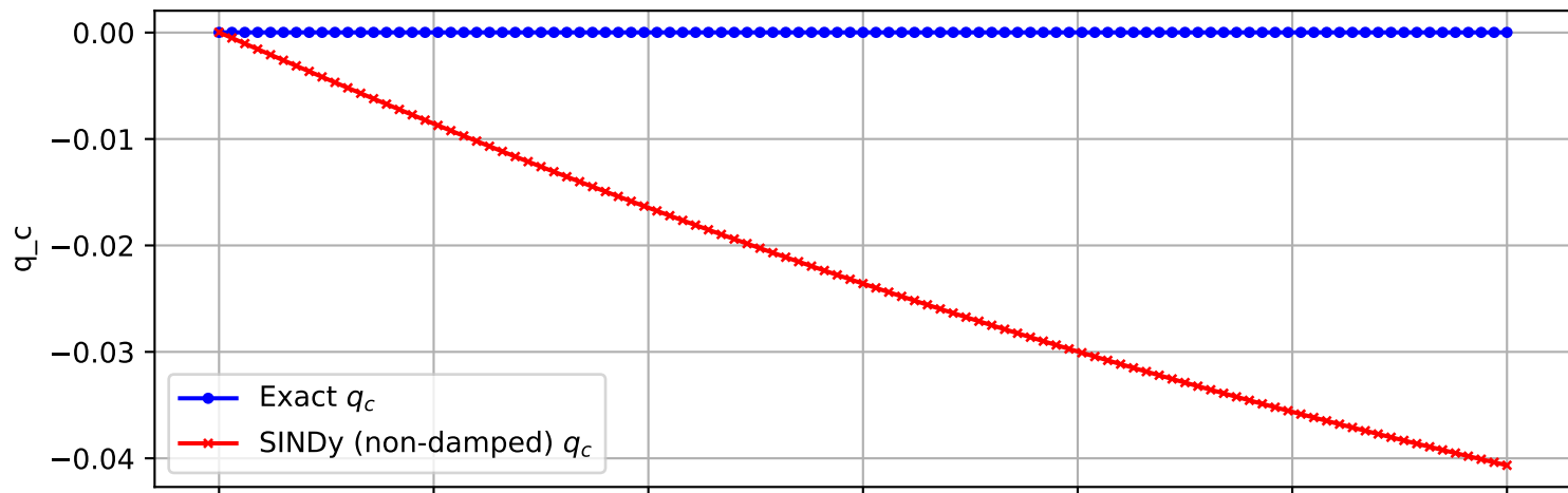
Trajectory 1927 (non-damped)
