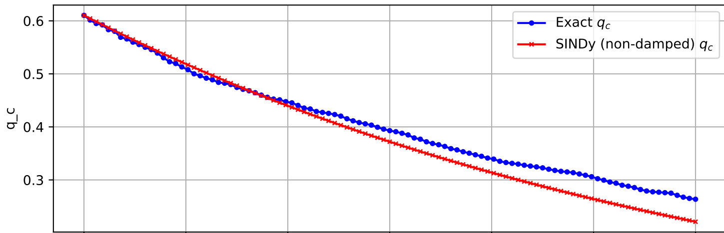
Trajectory 1929 (non-damped)
