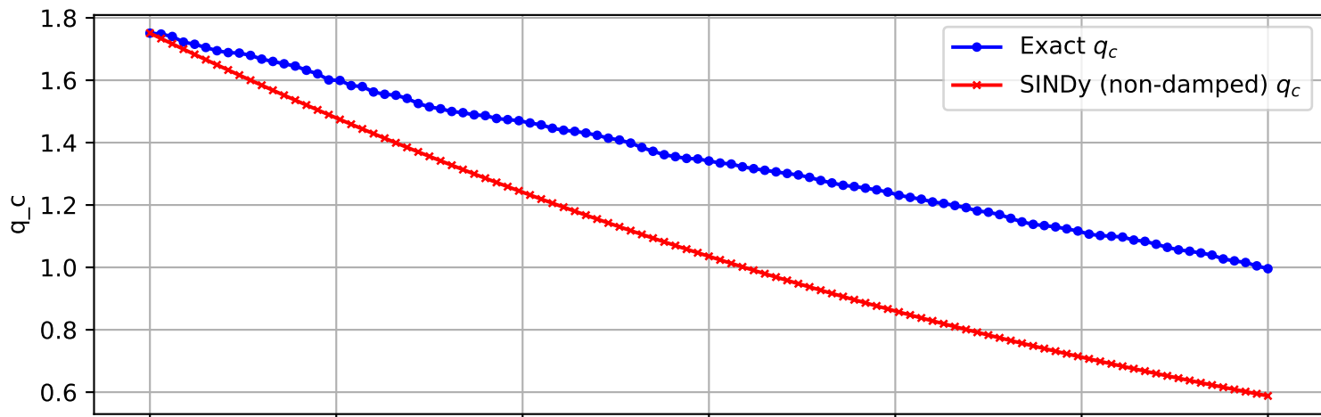
Trajectory 1930 (non-damped)
