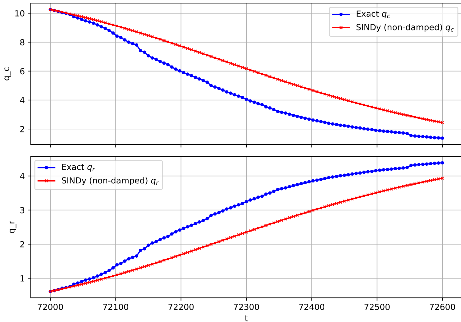
Trajectory 1932 (non-damped)
