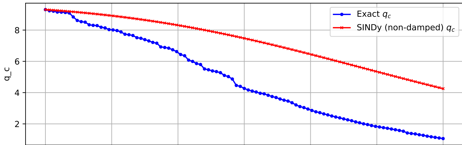
Trajectory 1933 (non-damped)
