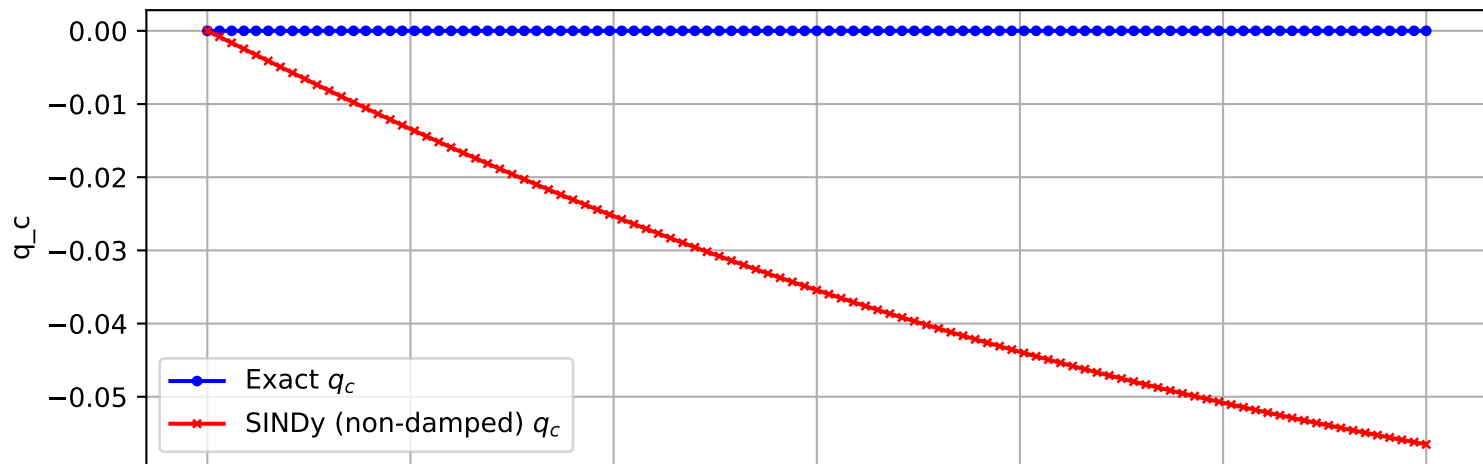
Trajectory 1937 (non-damped)
