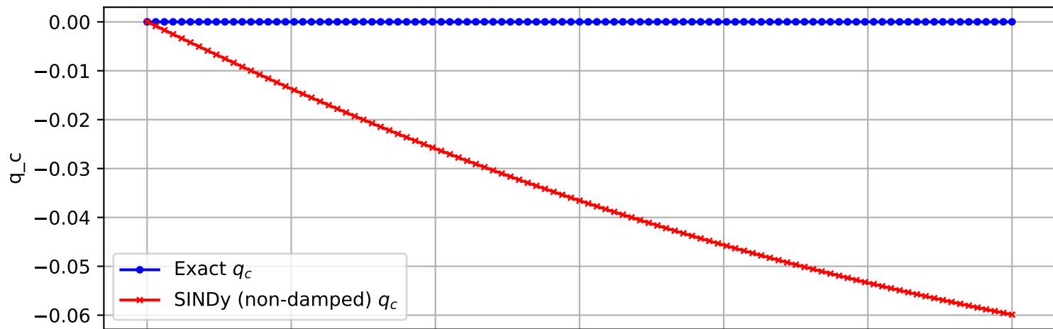
Trajectory 1941 (non-damped)
