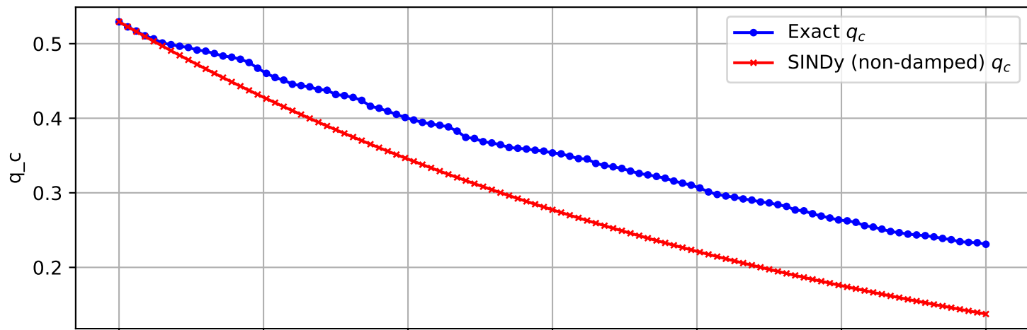
Trajectory 1946 (non-damped)
