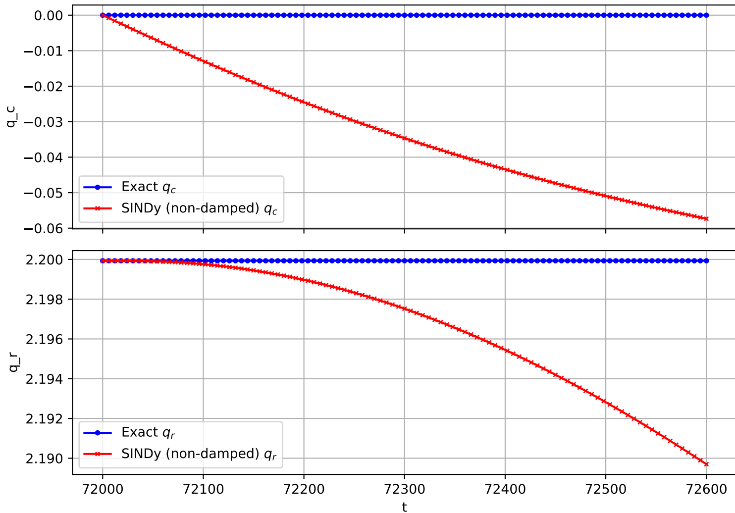
Trajectory 1953 (non-damped)
