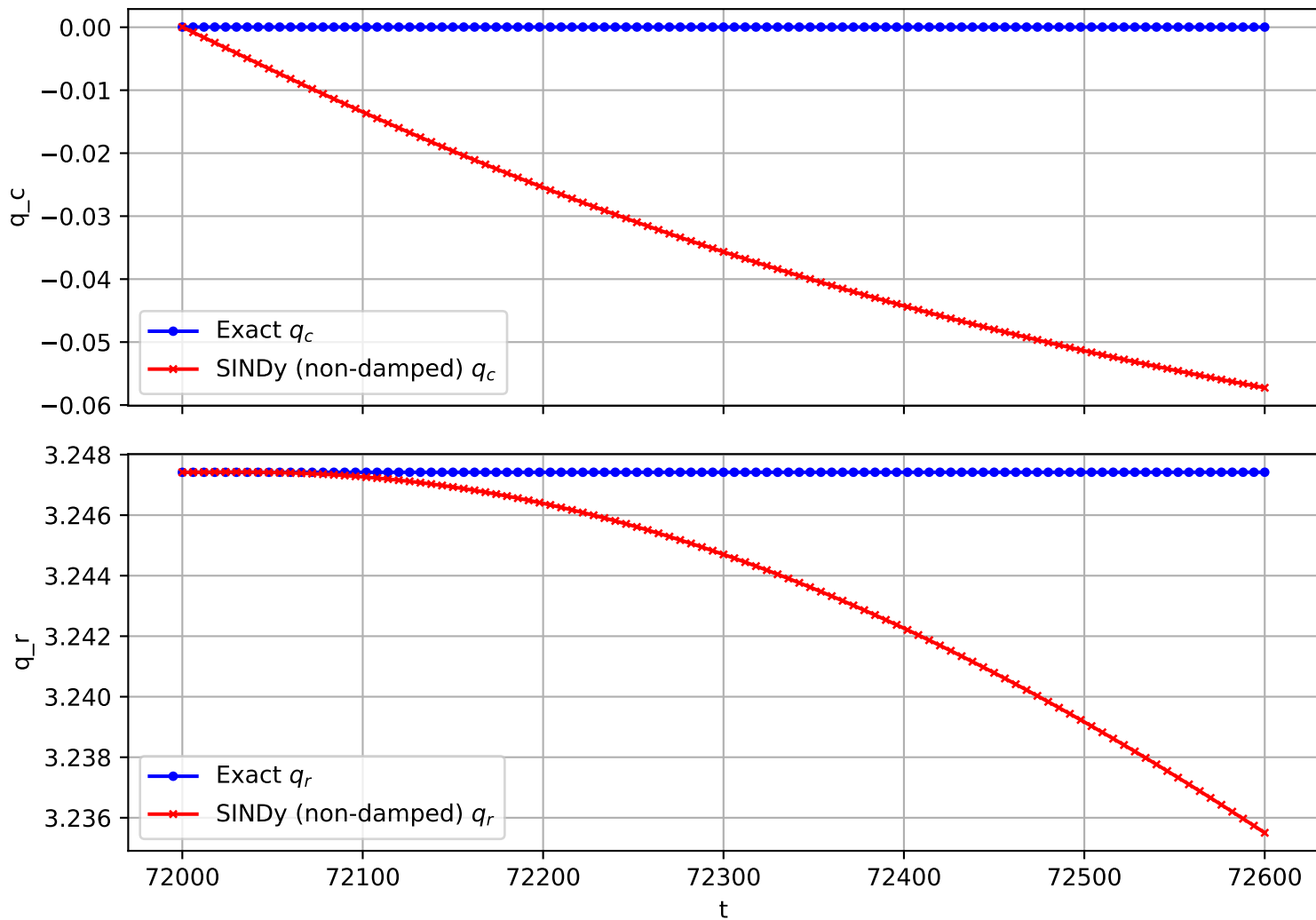
Trajectory 1959 (non-damped)
