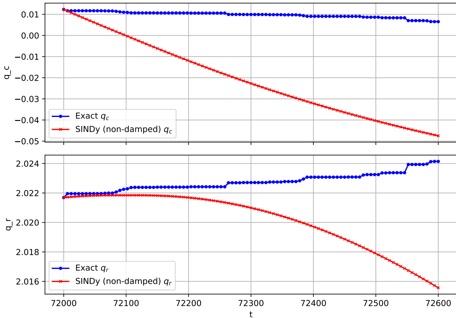
Trajectory 1962 (non-damped)
