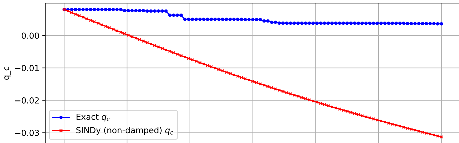
Trajectory 1963 (non-damped)
