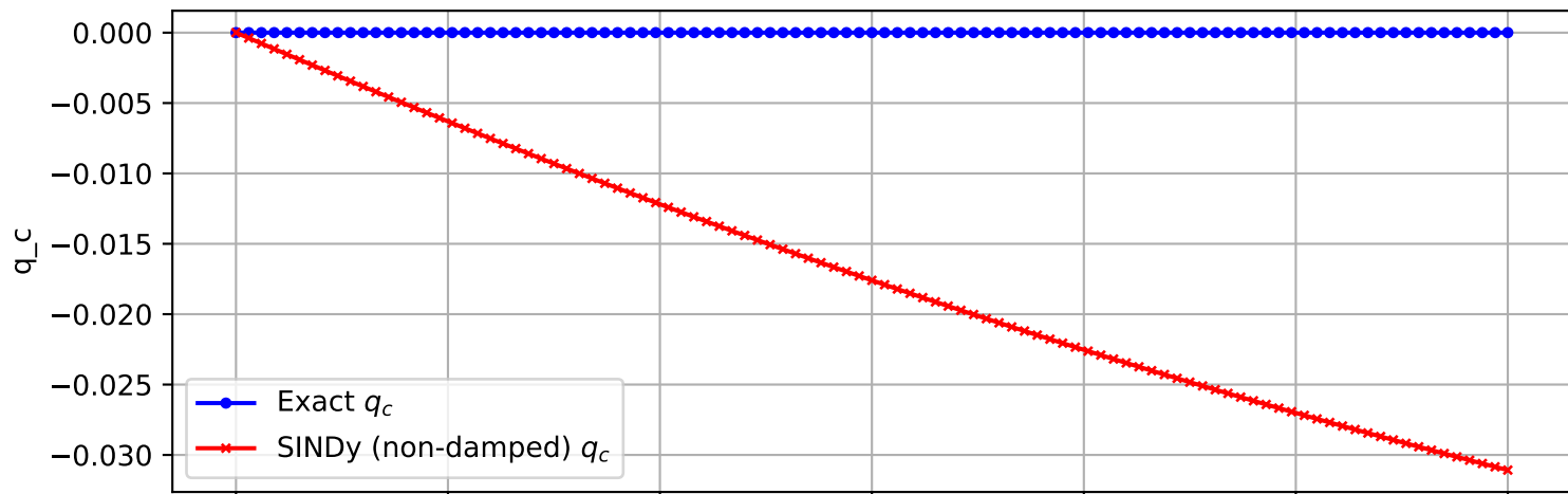
Trajectory 1972 (non-damped)
