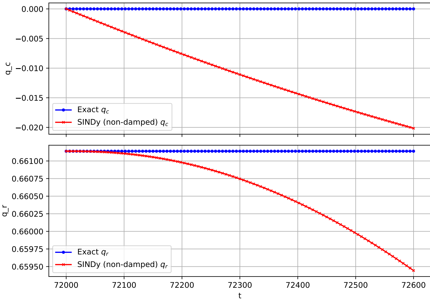
Trajectory 1980 (non-damped)
