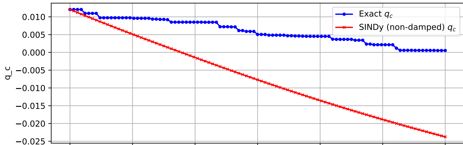
Trajectory 1982 (non-damped)
