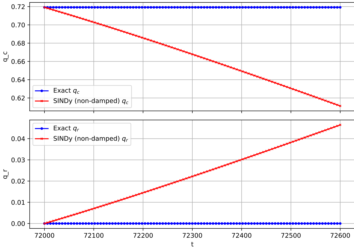
Trajectory 1994 (non-damped)
