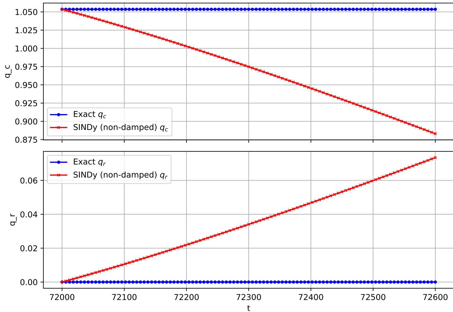
Trajectory 1995 (non-damped)
