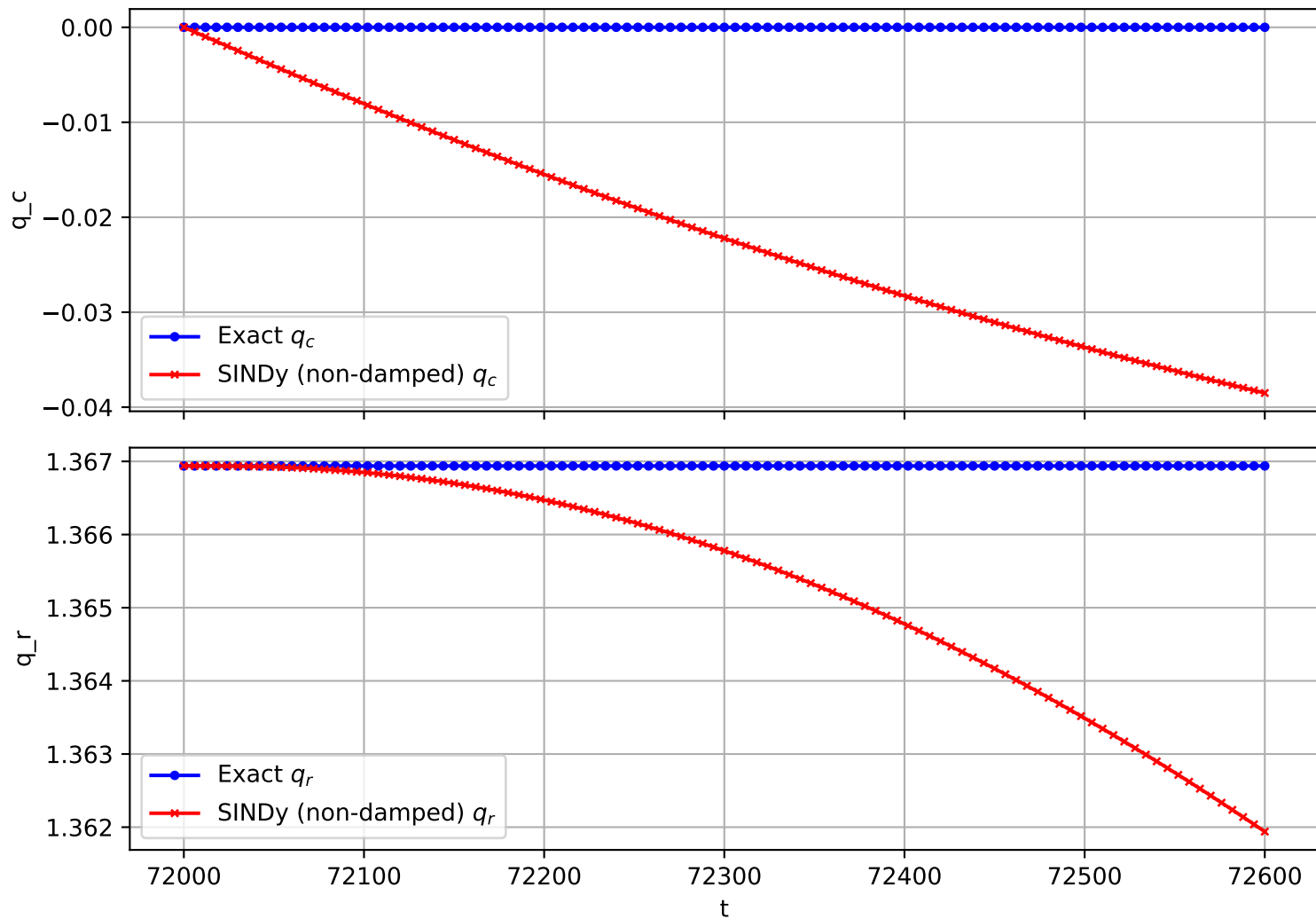
Trajectory 1998 (non-damped)
