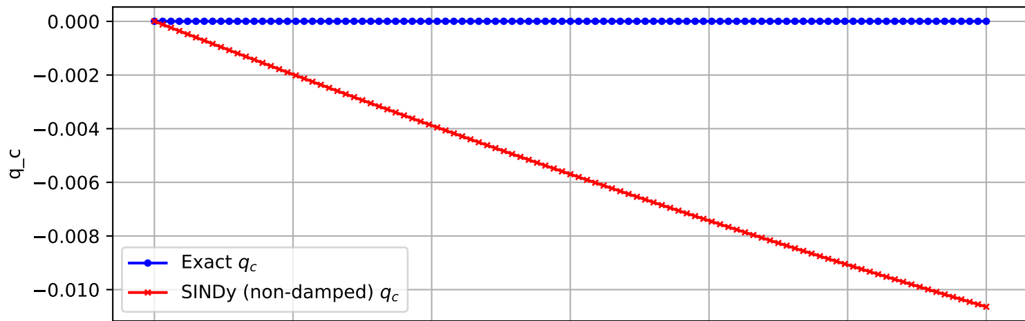
Trajectory 2031 (non-damped)
