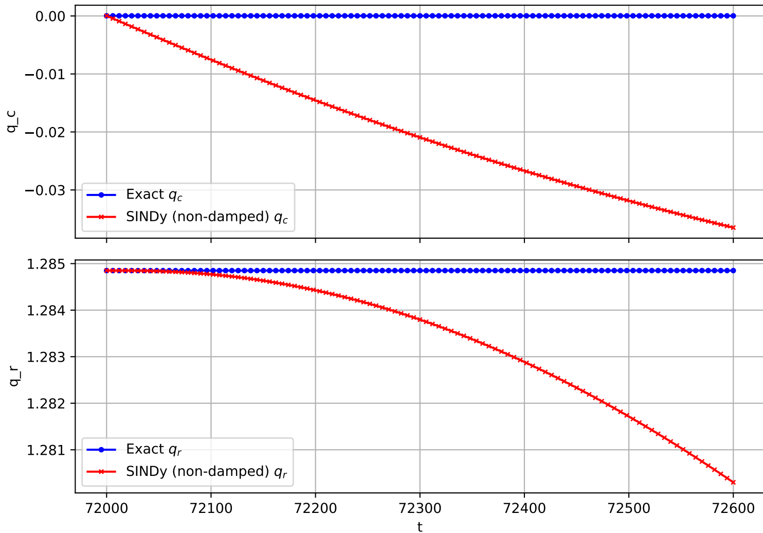
Trajectory 2035 (non-damped)
