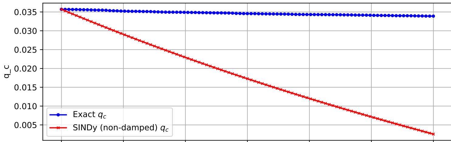
Trajectory 2036 (non-damped)
