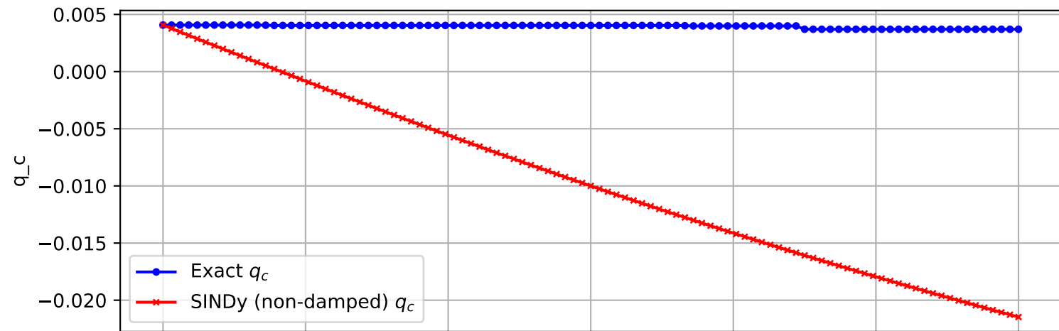
Trajectory 2039 (non-damped)
