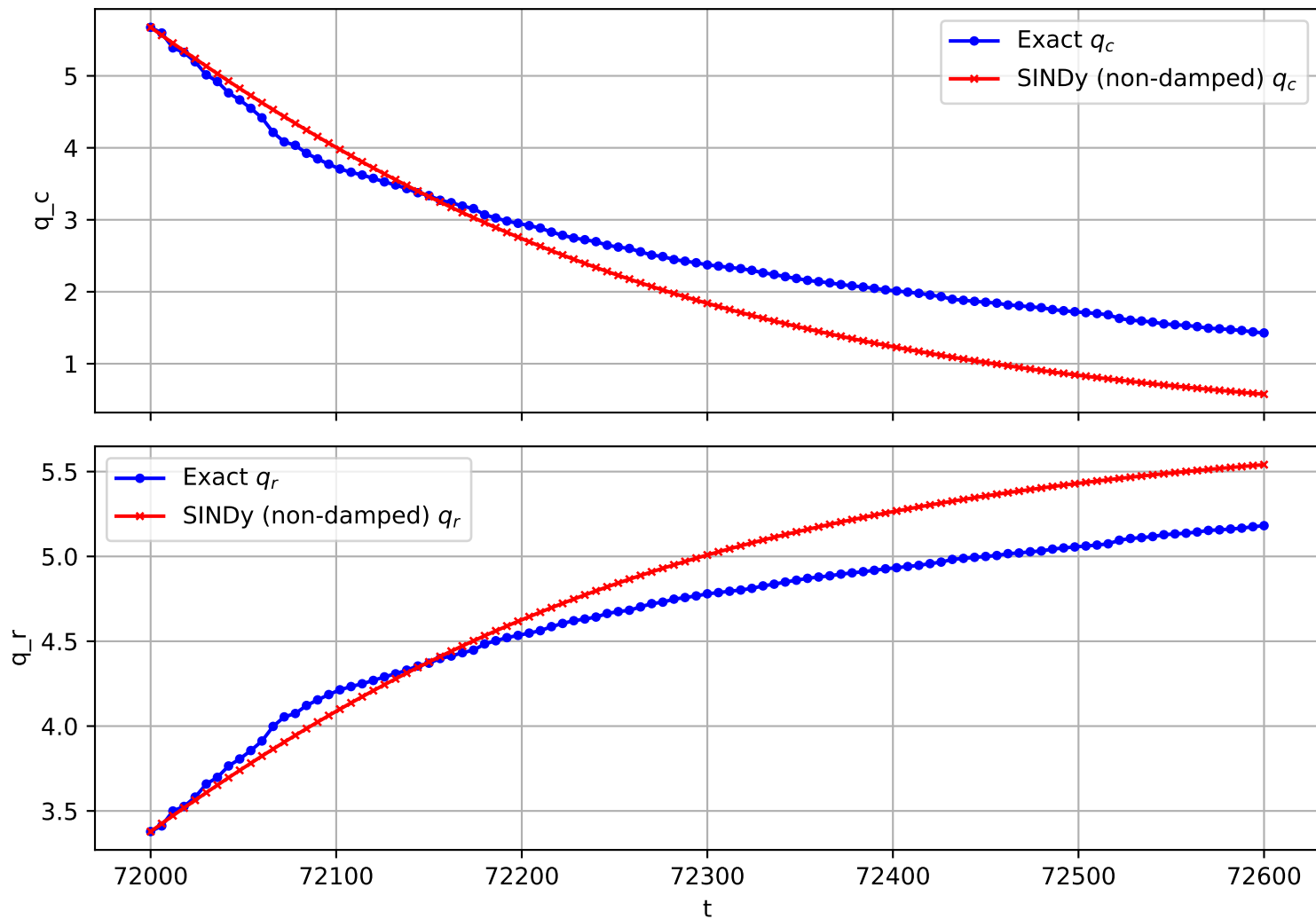
Trajectory 204 (non-damped)
