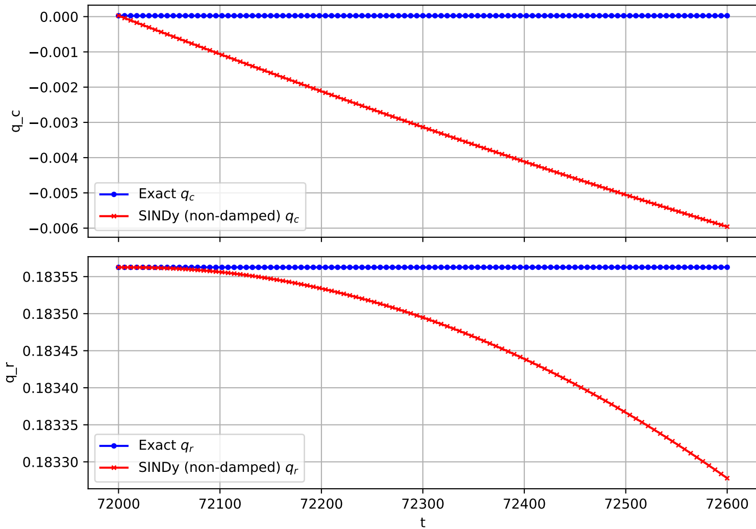
Trajectory 2049 (non-damped)
