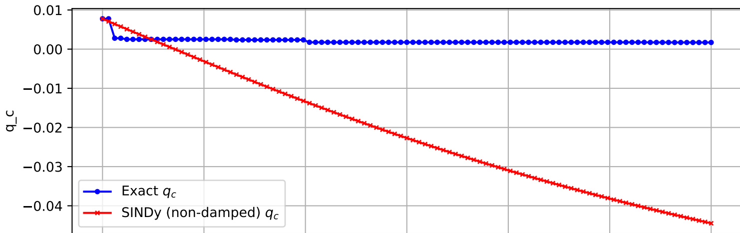
Trajectory 2057 (non-damped)
