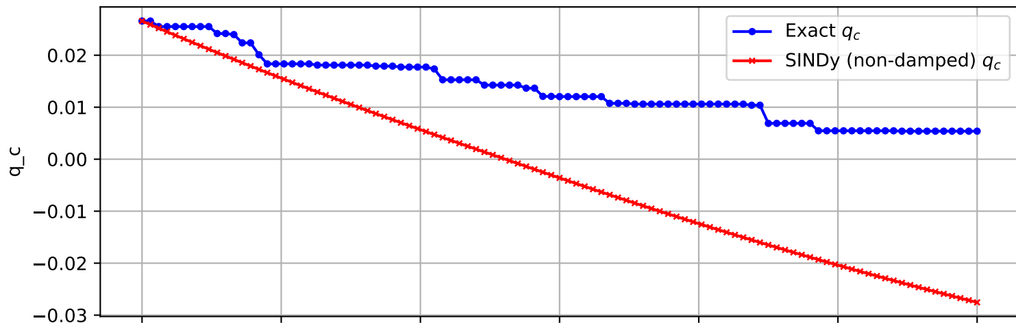
Trajectory 2062 (non-damped)
