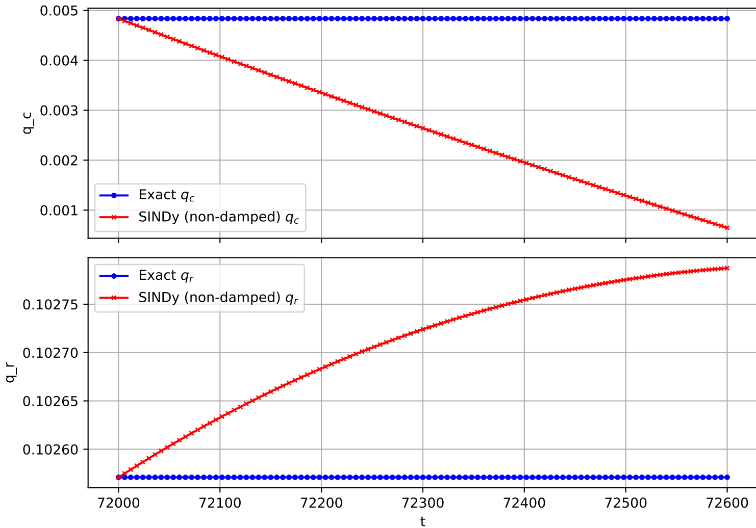
Trajectory 2074 (non-damped)
