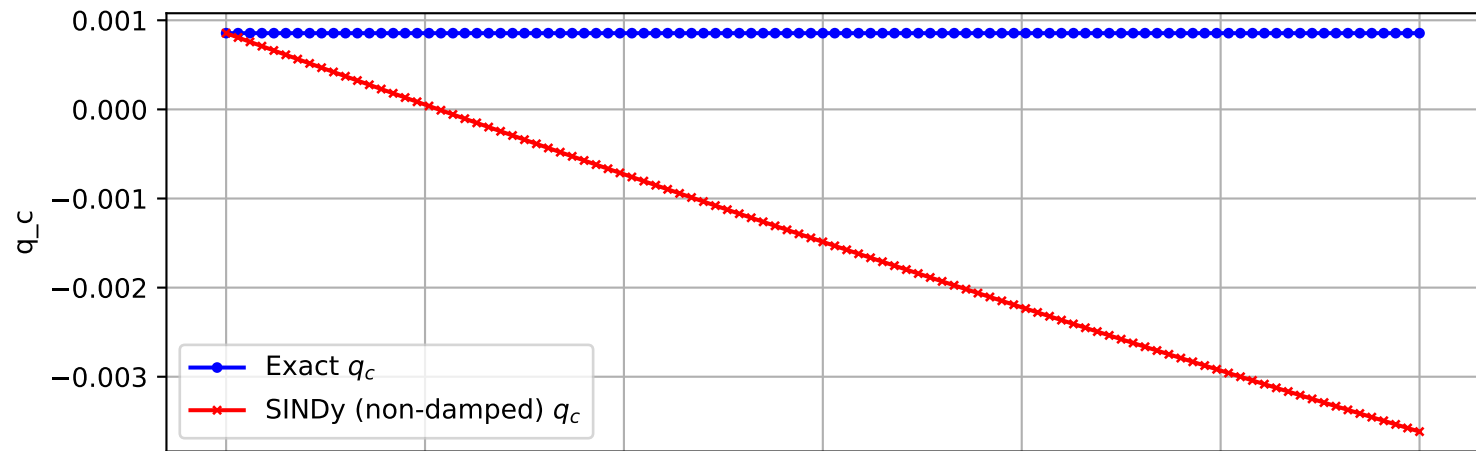
Trajectory 2076 (non-damped)
