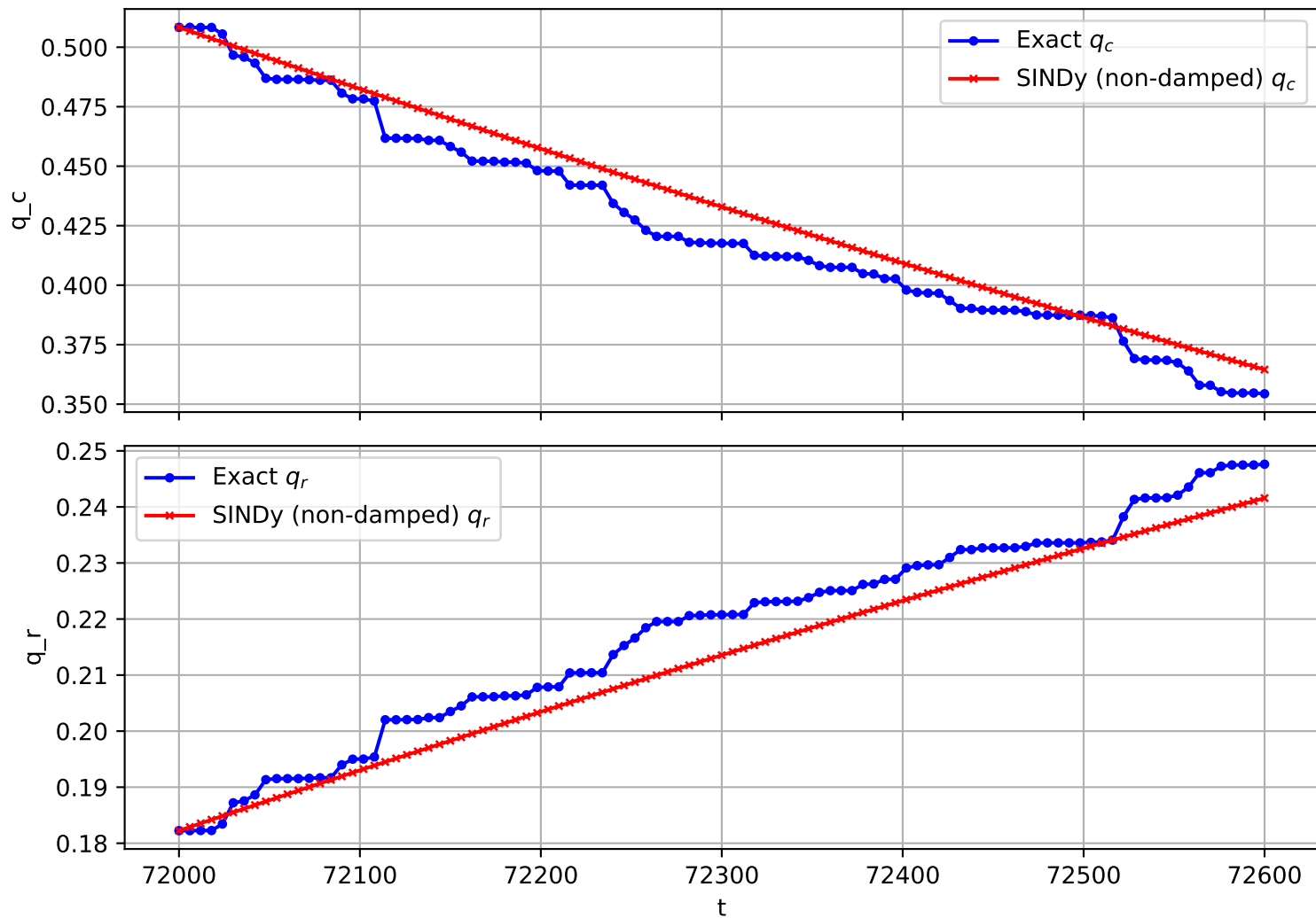
Trajectory 2086 (non-damped)
