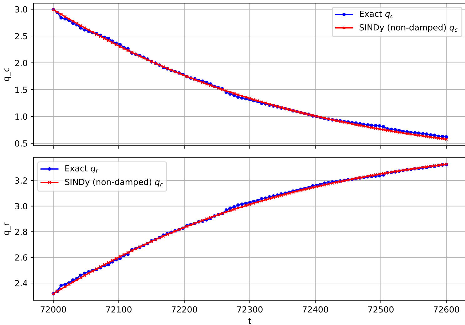
Trajectory 2089 (non-damped)
