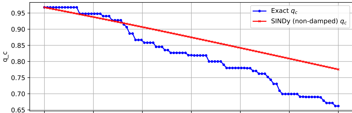
Trajectory 2093 (non-damped)
