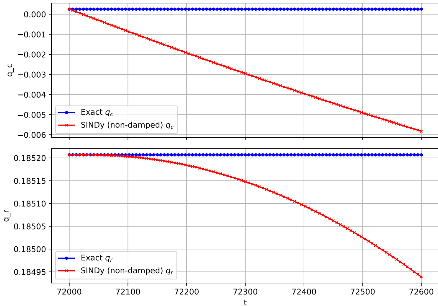
Trajectory 2096 (non-damped)
