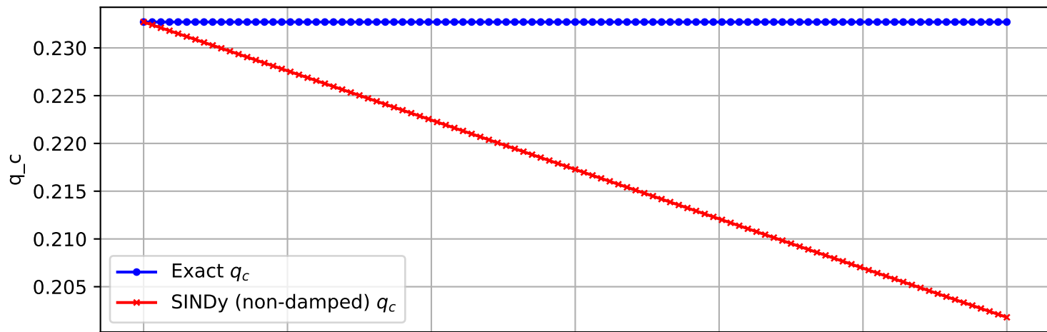
Trajectory 21 (non-damped)
