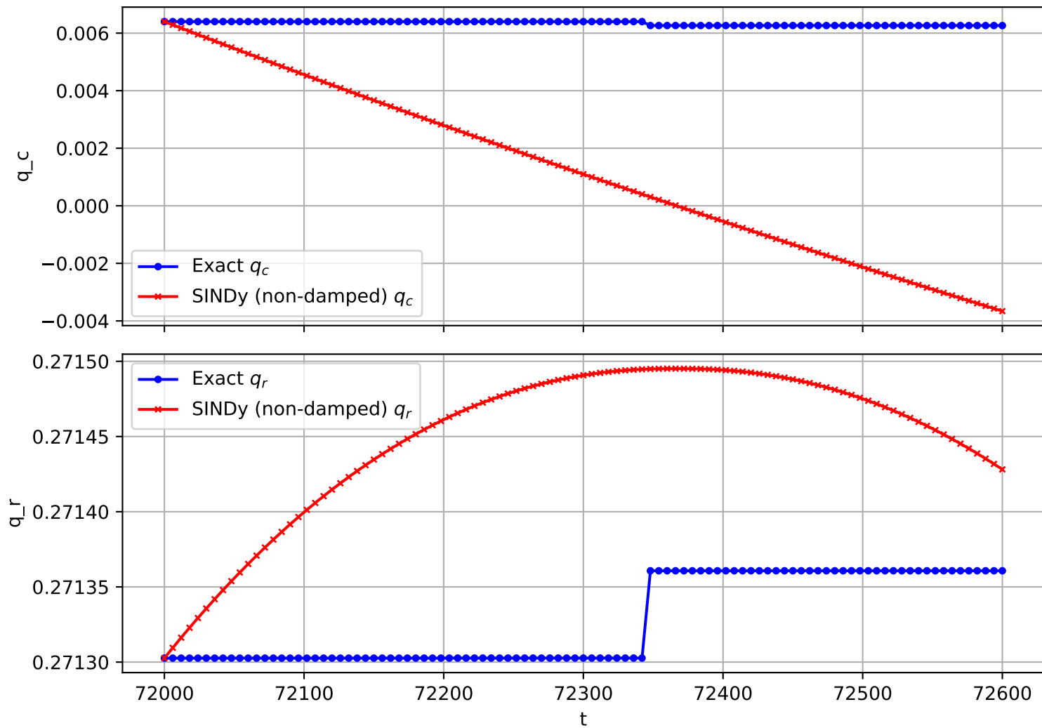
Trajectory 2101 (non-damped)
