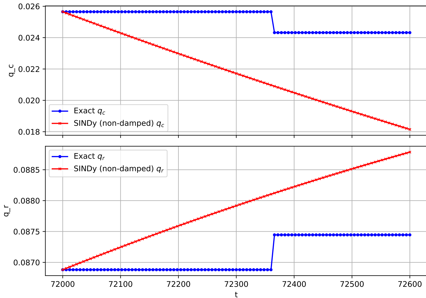
Trajectory 2108 (non-damped)
