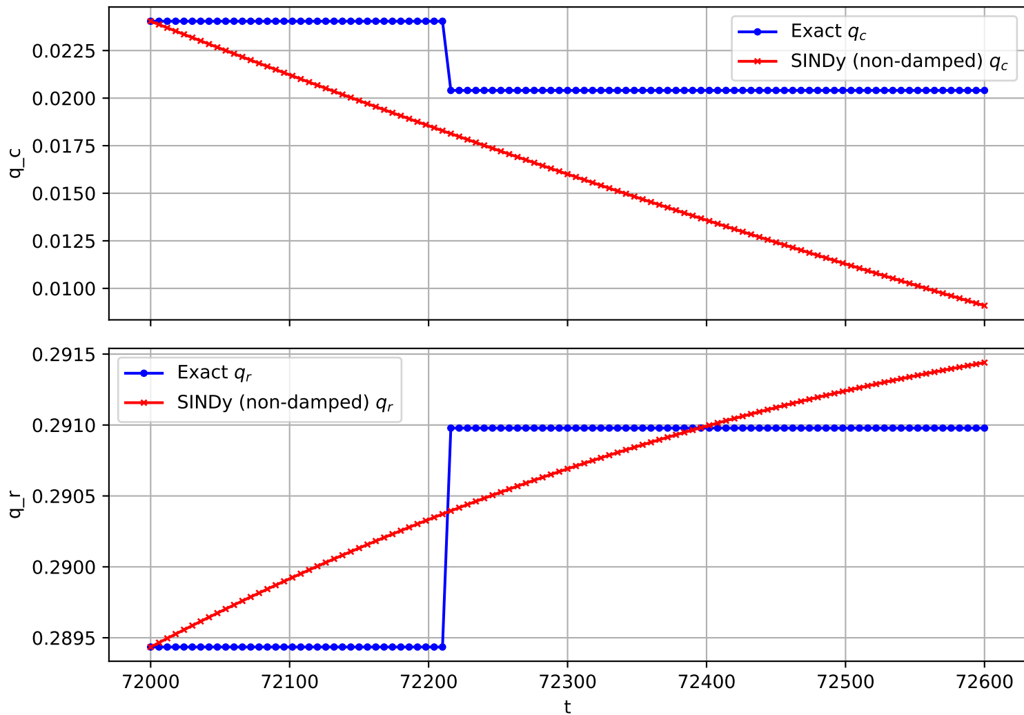
Trajectory 2114 (non-damped)
