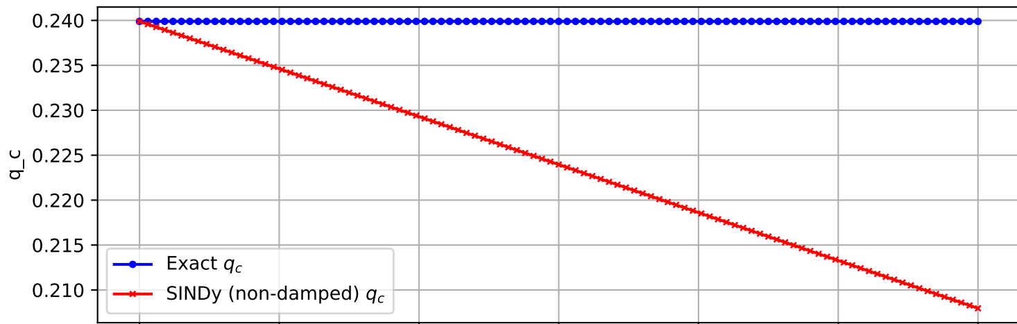
Trajectory 2116 (non-damped)
