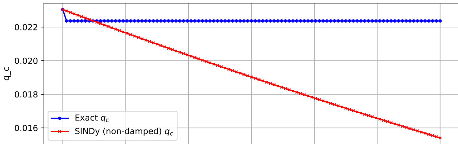
Trajectory 2117 (non-damped)
