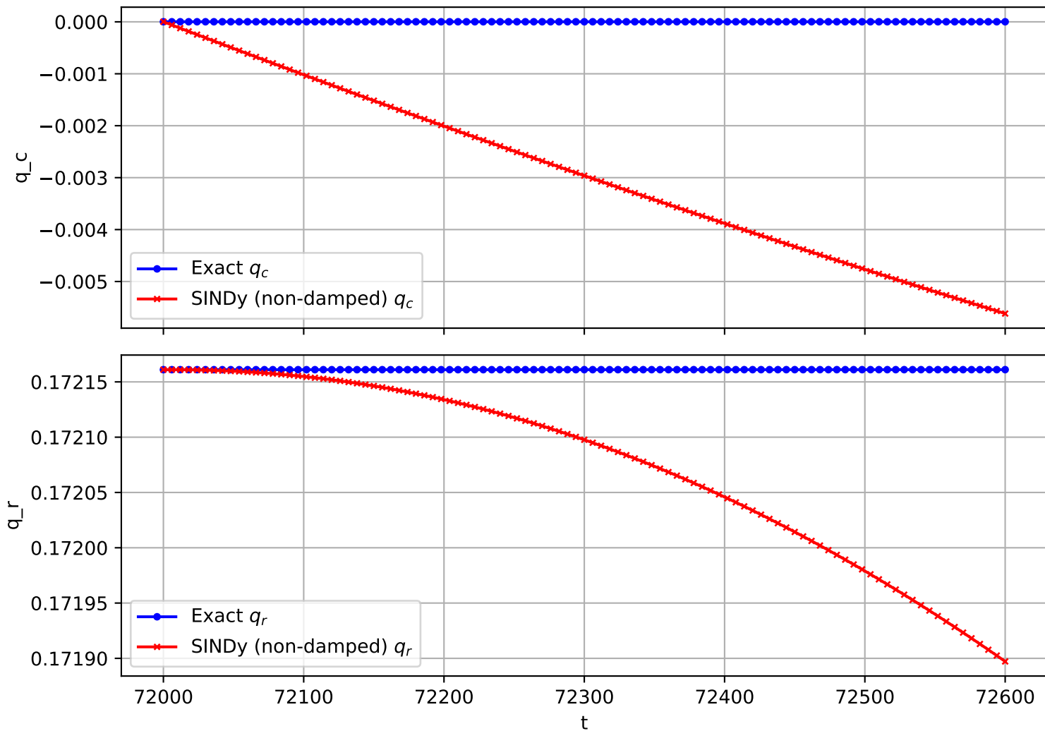
Trajectory 2124 (non-damped)
