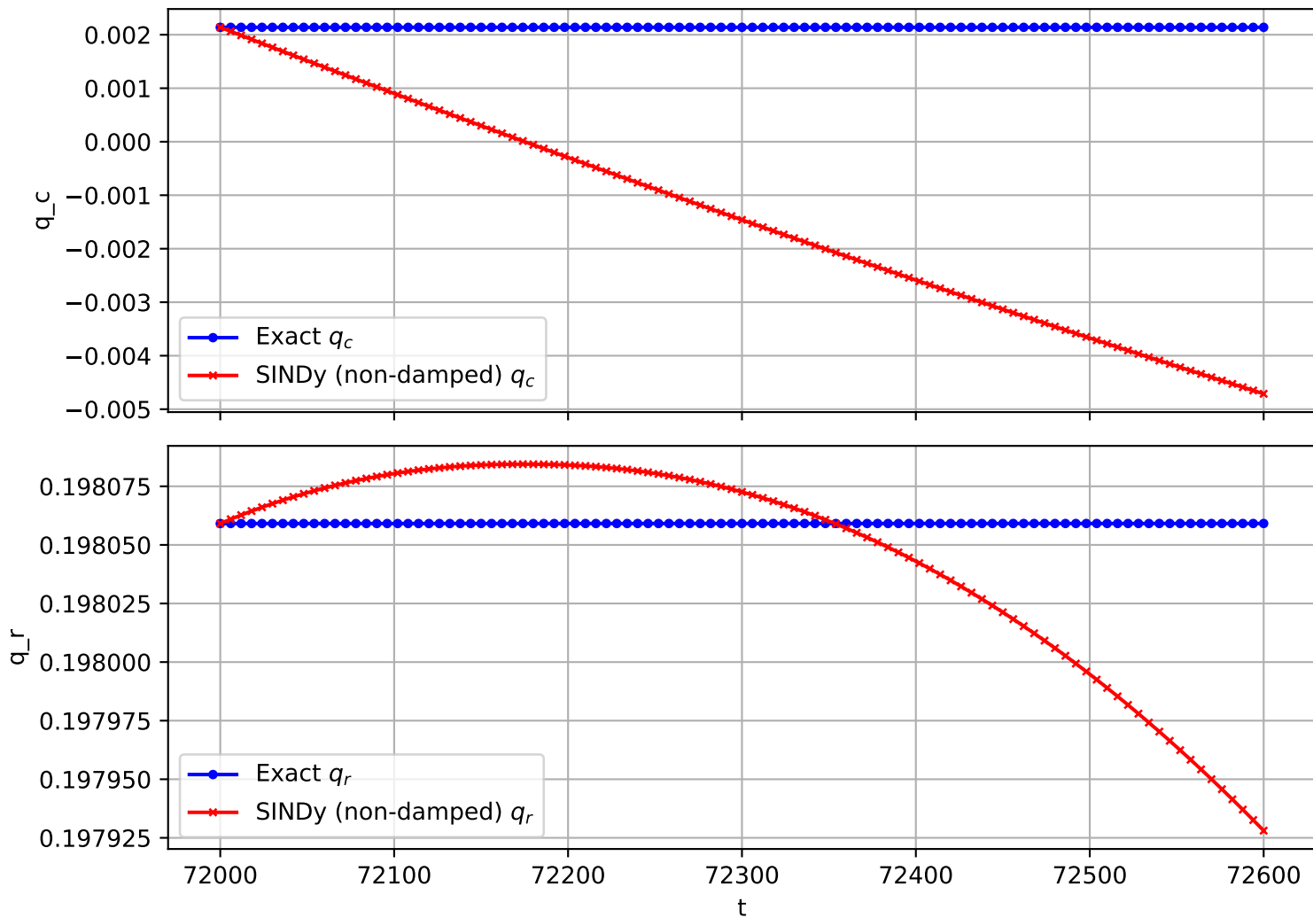
Trajectory 2130 (non-damped)
