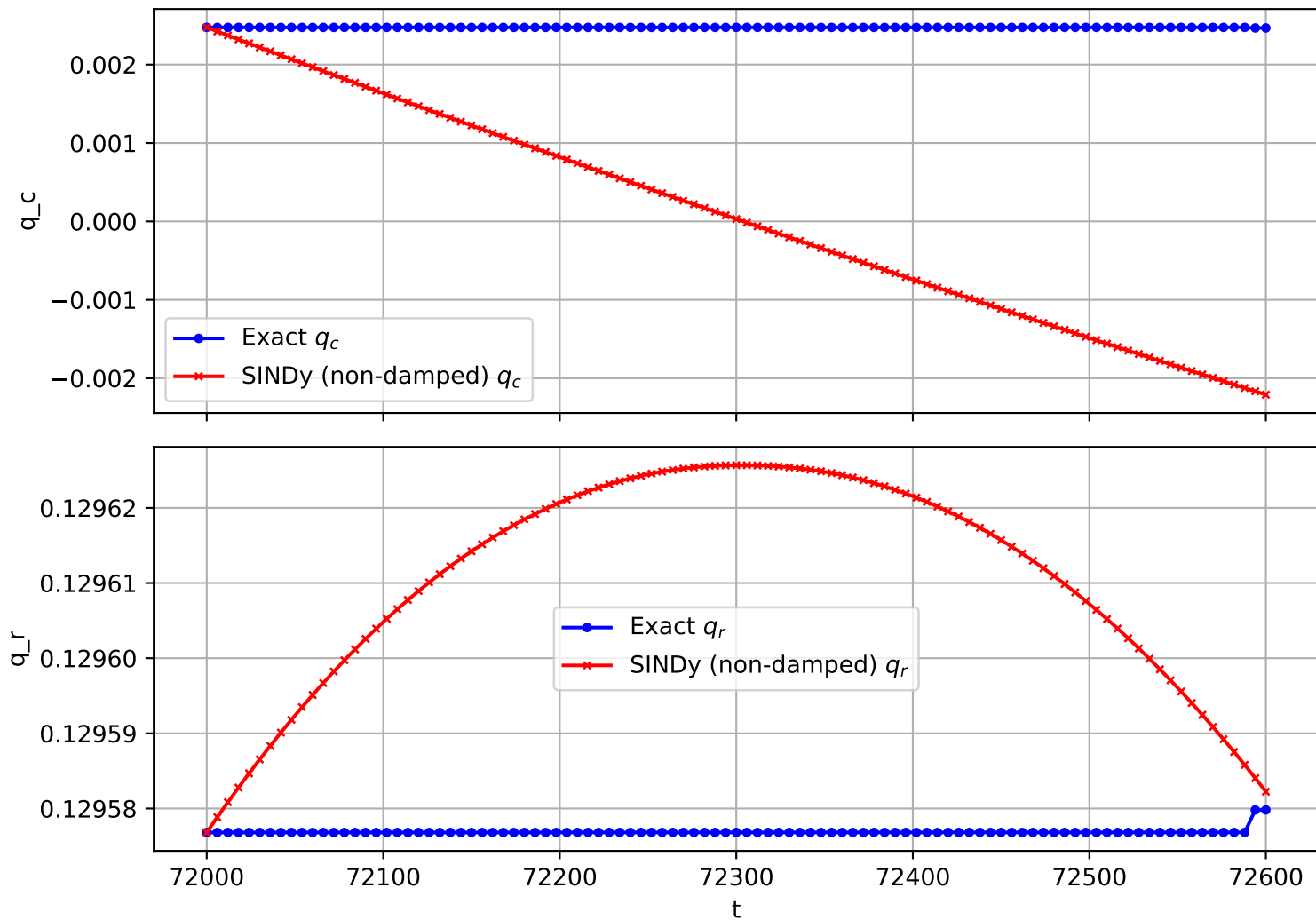
Trajectory 2131 (non-damped)
