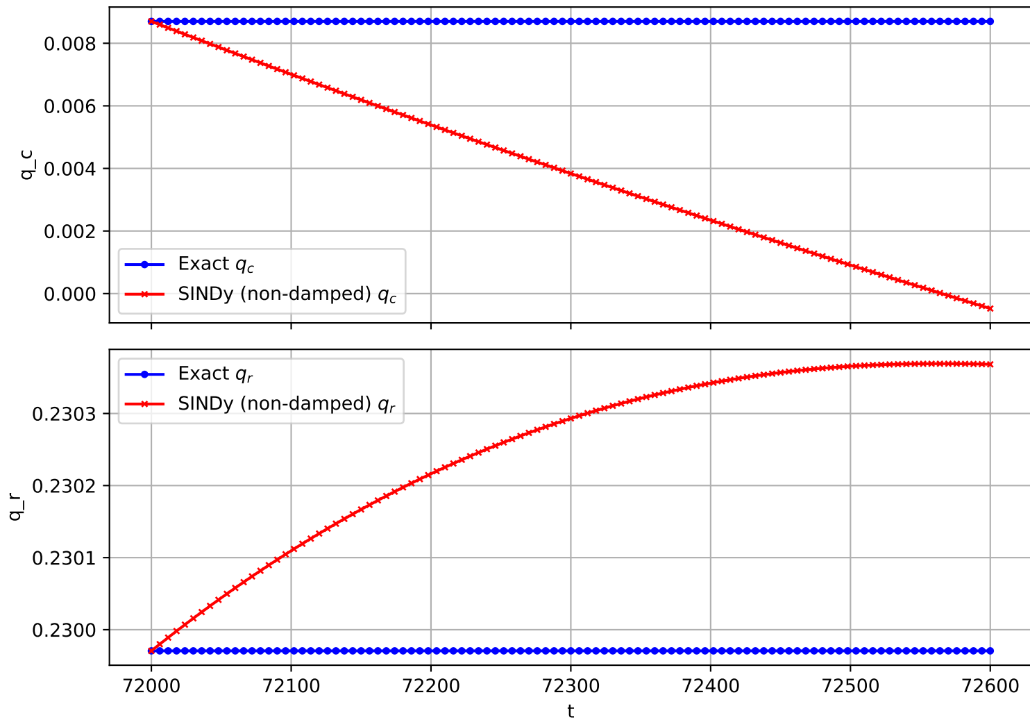
Trajectory 2135 (non-damped)
