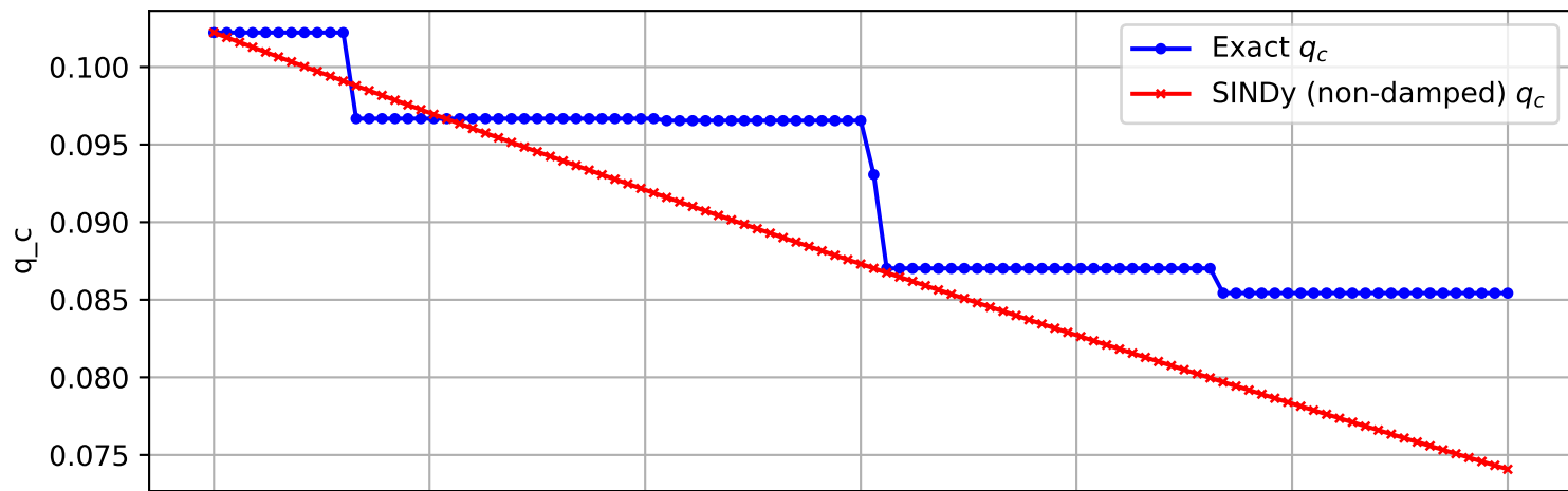
Trajectory 2137 (non-damped)
